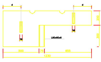
PRECAST COVER TYPE (C1) Sc. 1:10
